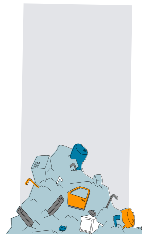
Sucata 26.707 kg
